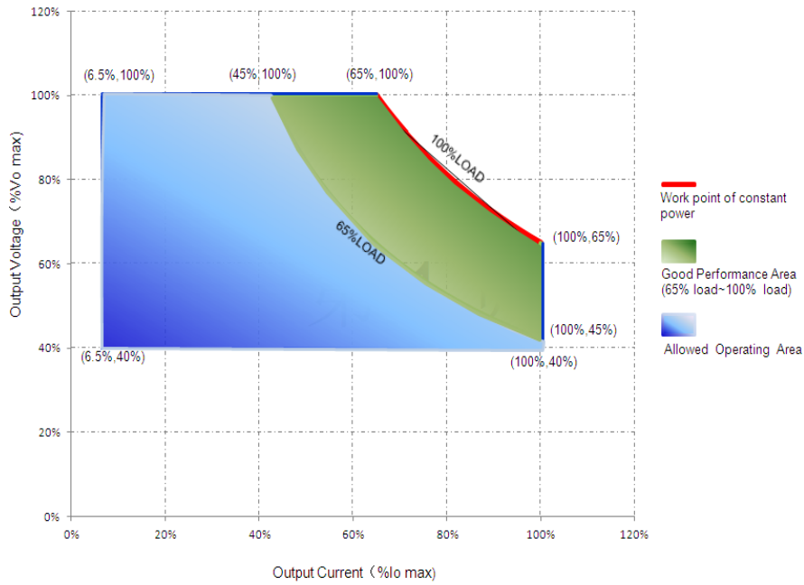
V/I Operating Area
